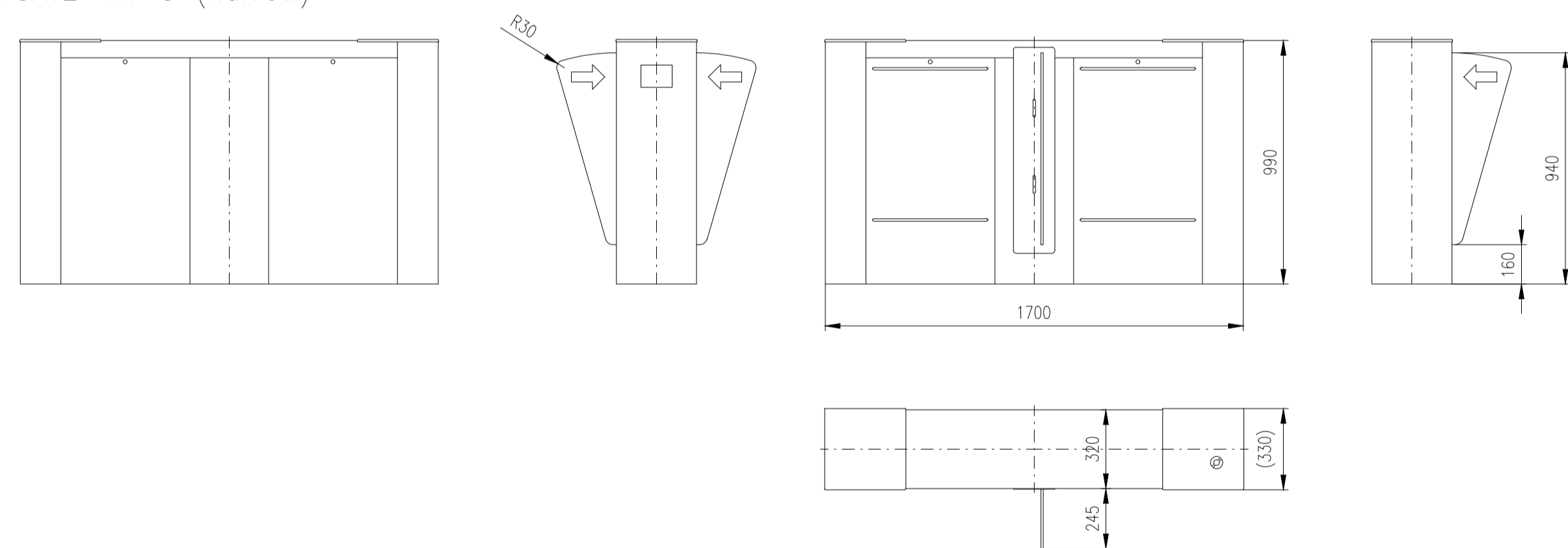
Turnstile: EASYGATE-FHI-S
