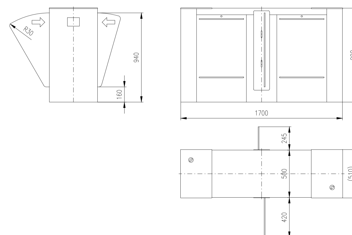
Turnstile: EASYGATE-FHI-M (wide/narrow)
